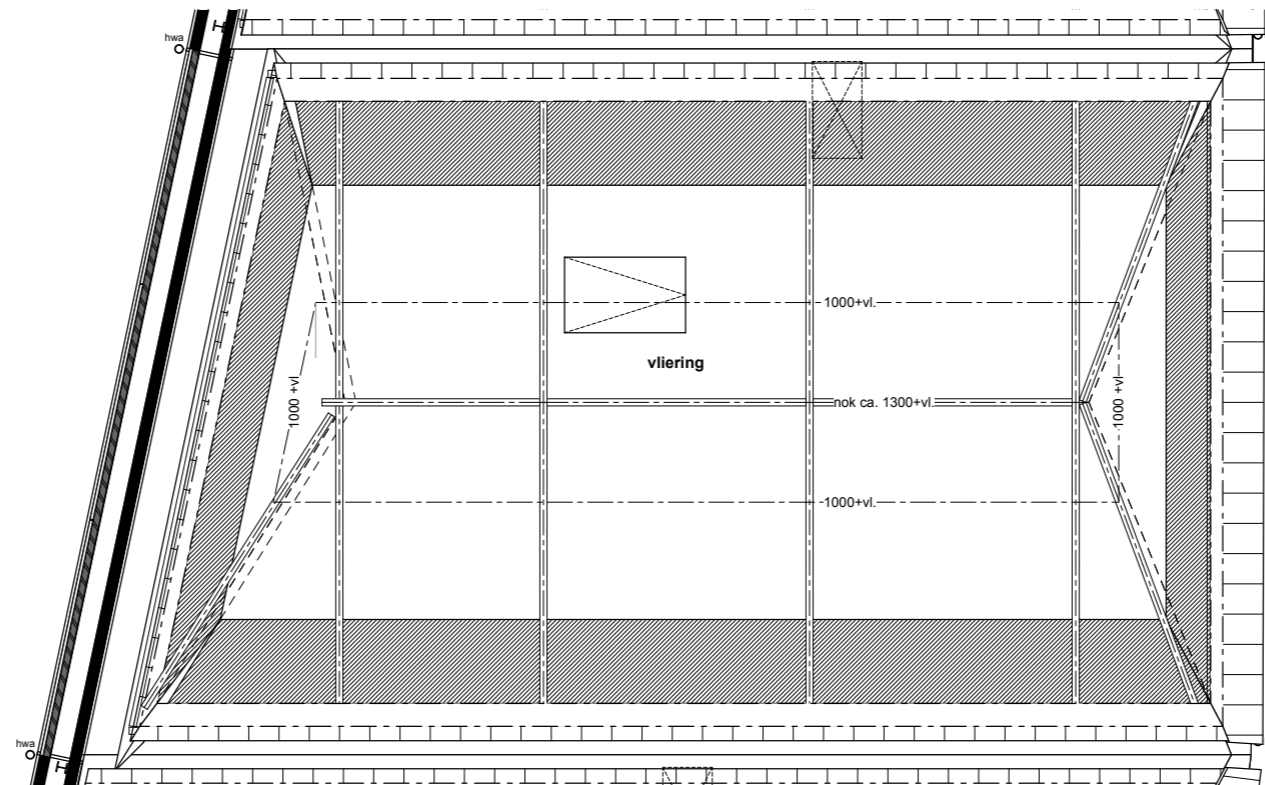
Bergzolder
